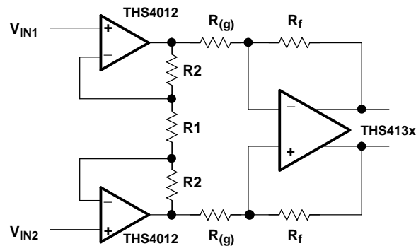
Figure 40. Instrumentation Amplifier
