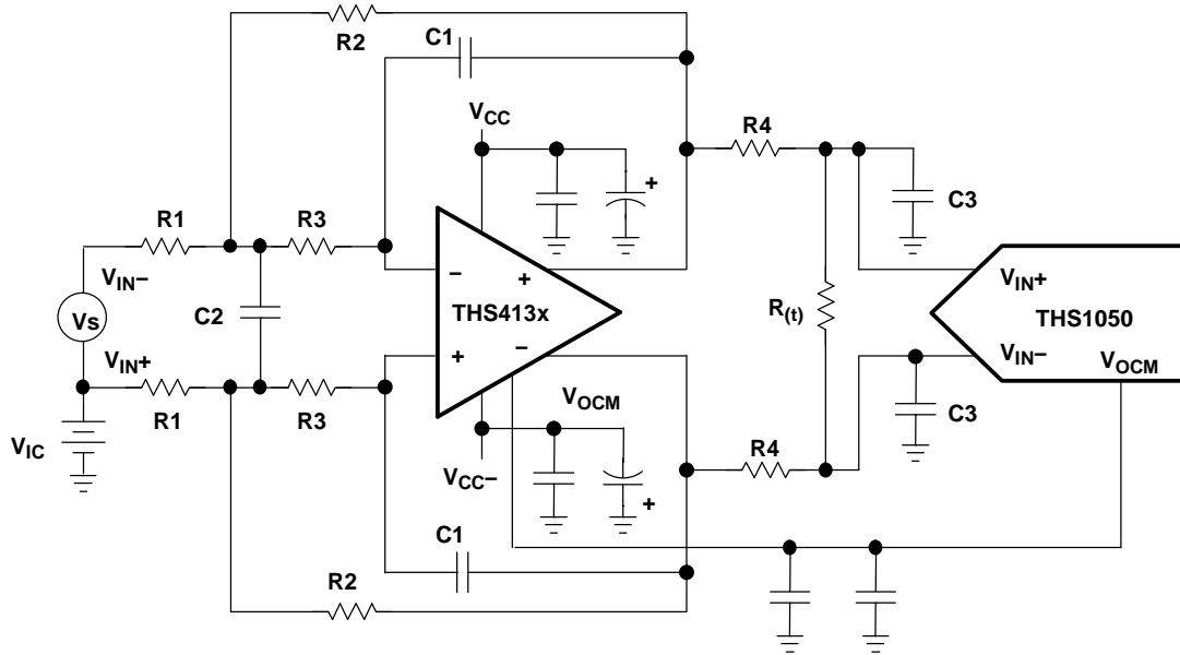
Figure 34. Antialias Filtering
